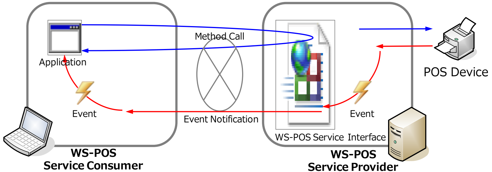
Figure 15: Method Call with Event Notification
