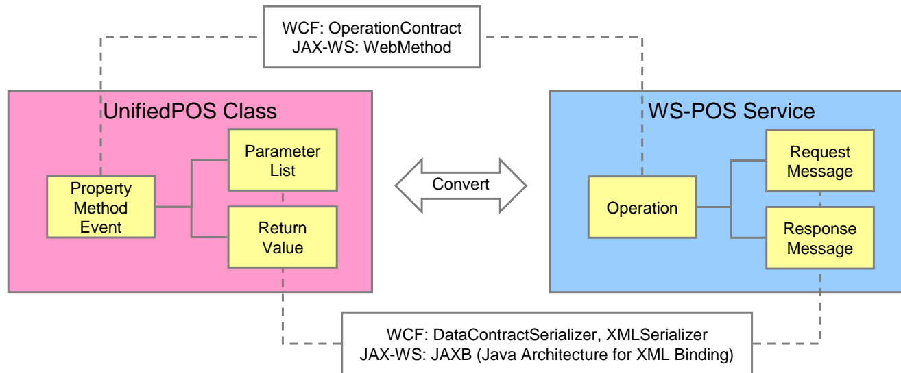
Figure 37: UnifiedPOS and WSDL Mapping
