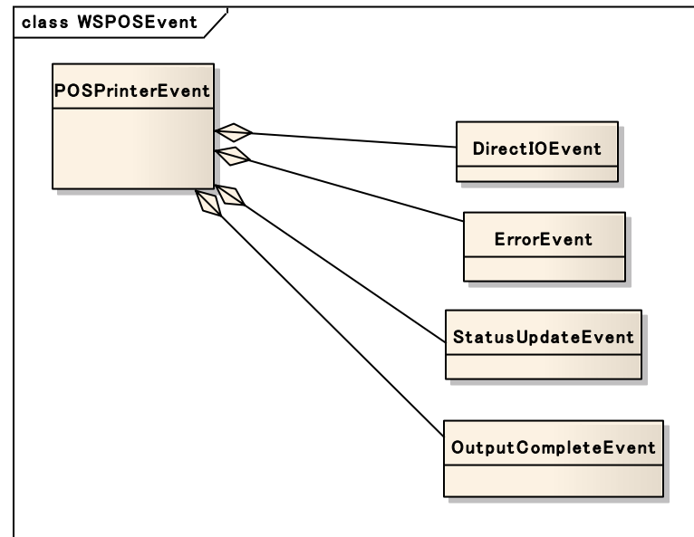
Figure 29: WSPOS POS Printer Event
