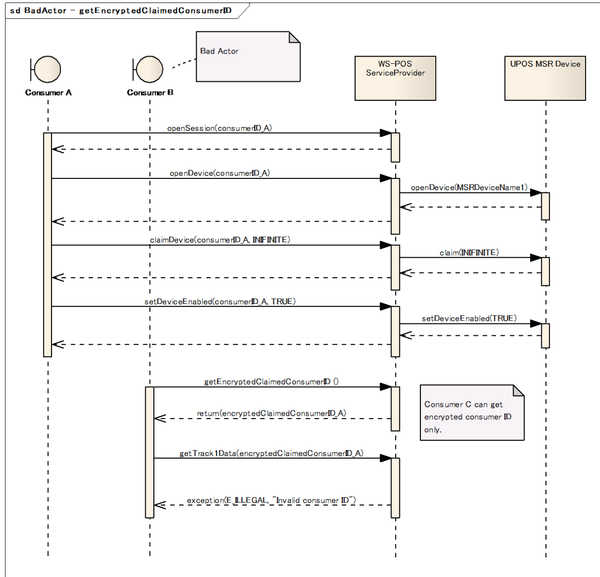
Figure 34: Get Encrypted Claimed Consumer ID
