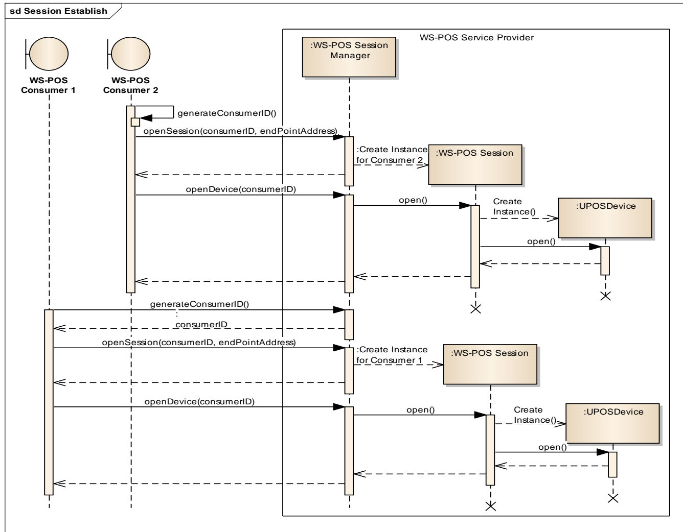
Figure 9: Establish Session
