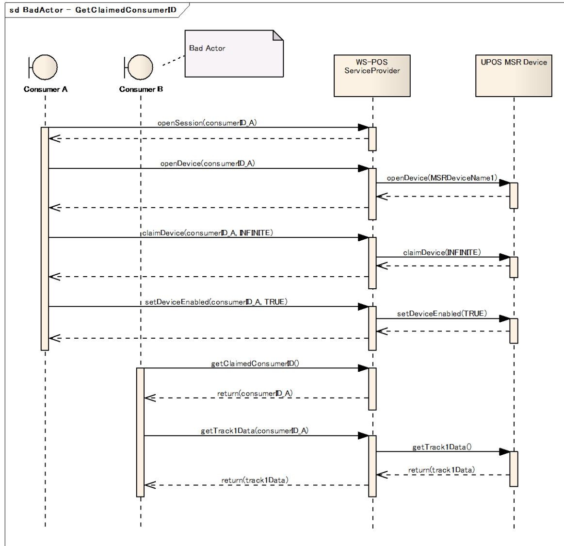
Figure 33: Get Claimed Consumer ID
