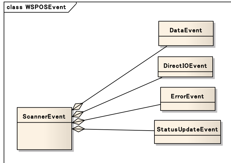
Figure 30: WSPOS - Scanner Event
