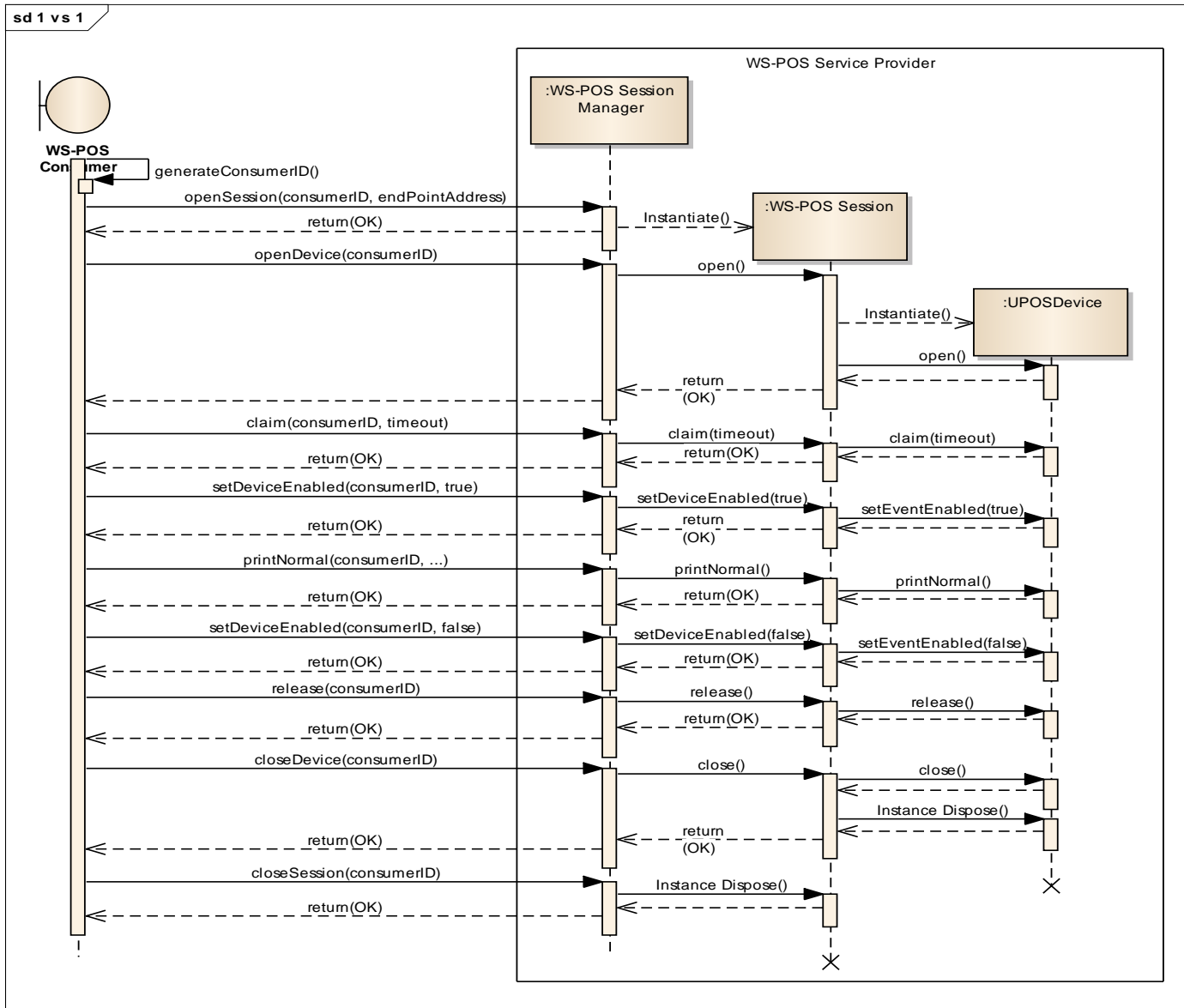
Figure 10: POS Printer - Print Normal example
