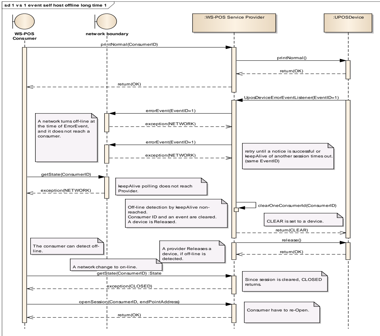
Figure 24: Offline Longer than Session Time Out in Bi-Directional Communication 1
