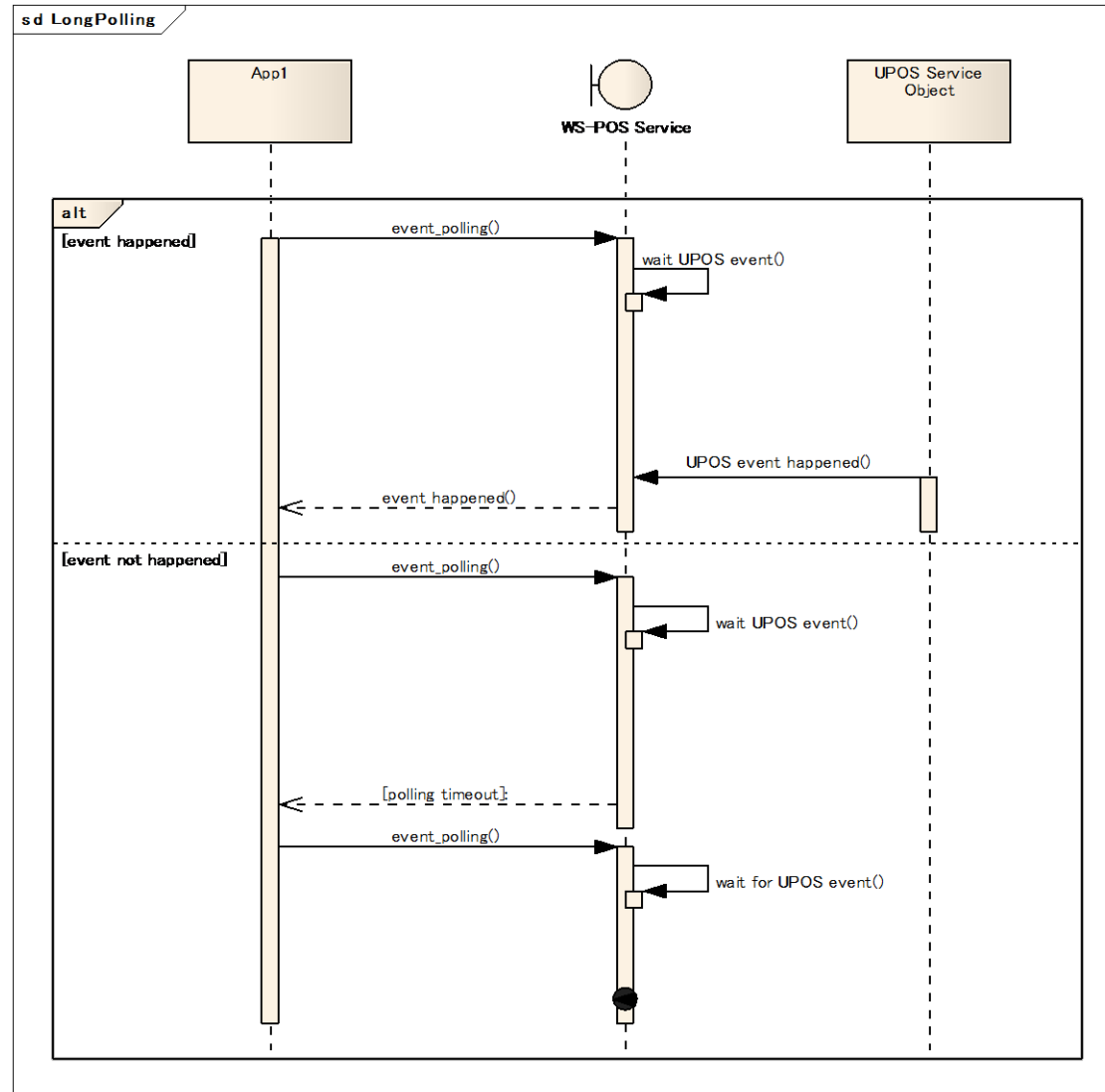
Figure 20: Long Polling
