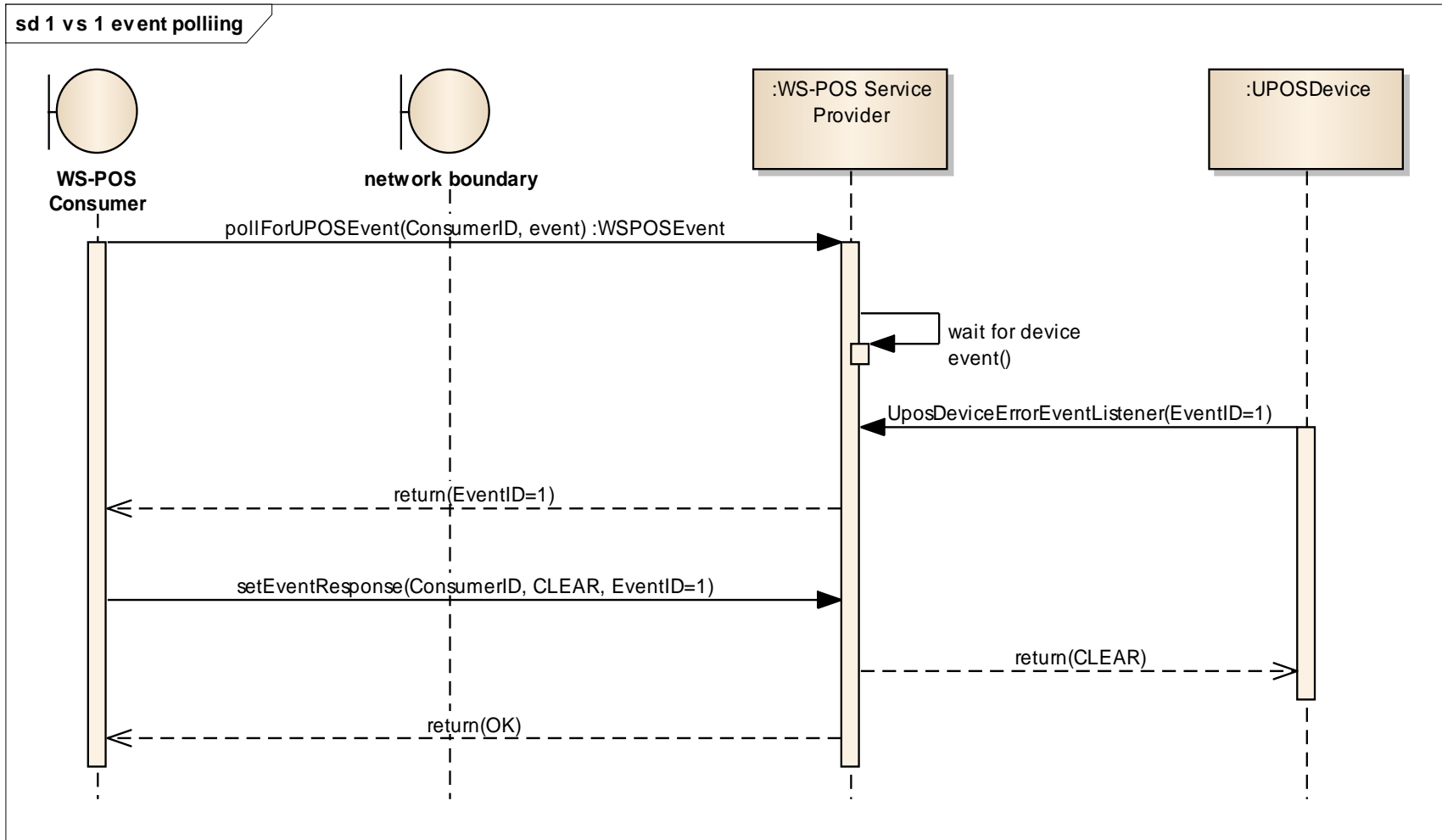
Figure 17: Event Polling
