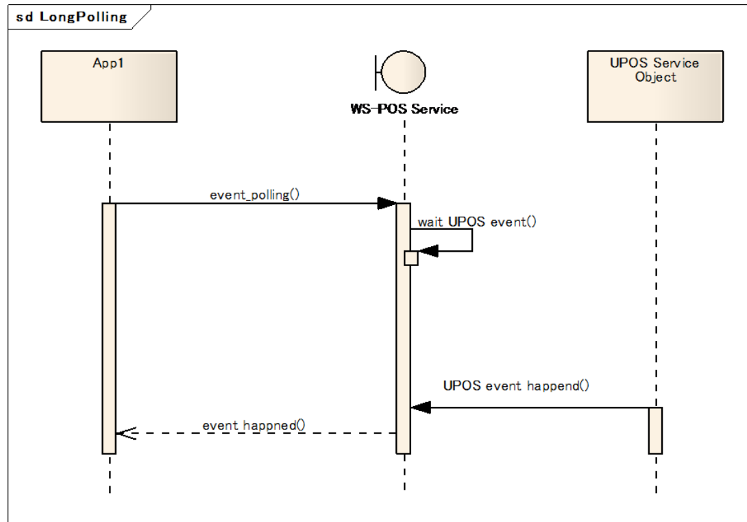
Figure 19: Long Polling Overview
