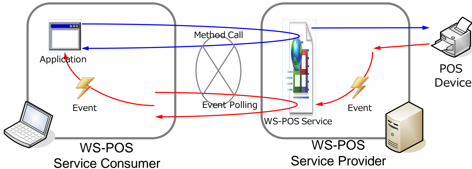
Figure 18 Method call and Event notification
