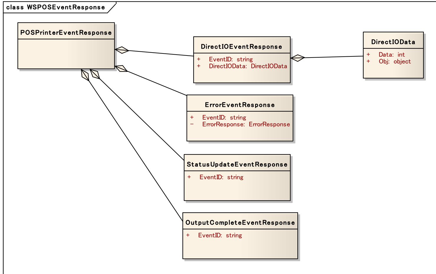
Figure 31: WSPOS Event Response
