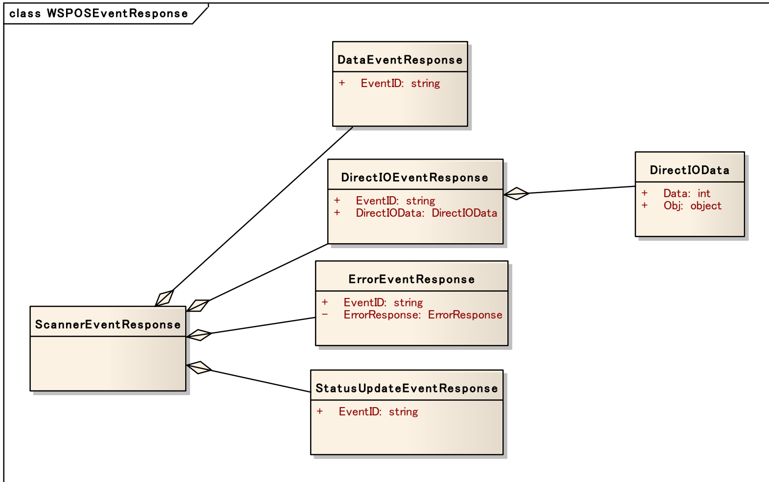
Figure 32: WSPOS - Event Response
