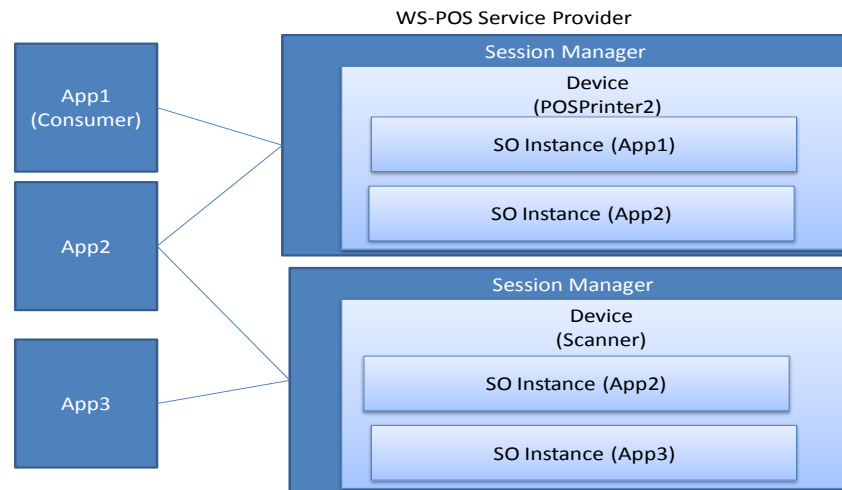
Figure 6: Session Management layer and Device Control layer
