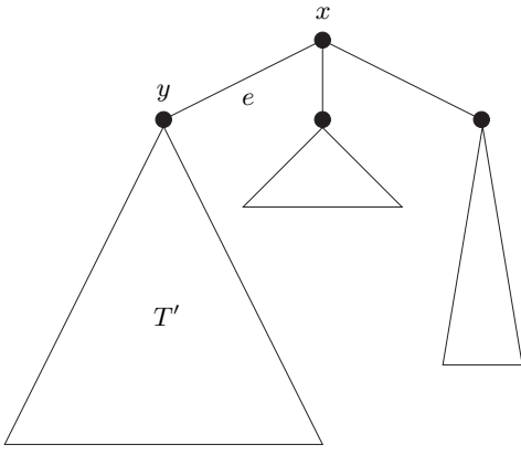
Figure 1. A finite tree T .
