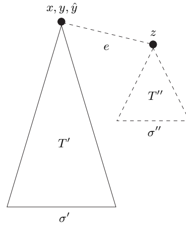
Figure 2. Tree T after the Add-Merge of T' and T'' . The dashed subtree is \hat{T} .
