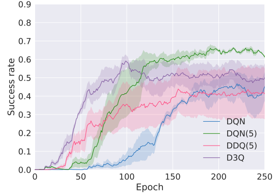
Figure 8: The learning curves of agents (DQN, DDQ, and D3Q) under the domain extension setting.
