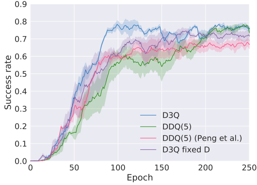
Figure 7: The learning curves of D3Q, DDQ(5), DDQ(5) (Peng et al., 2018), and D3Q fixed \theta_D agents.
