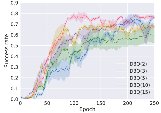
Figure 6: The Learning curves of D3Q( K ) agents which ( K-1 ) is the number of planning steps ( K = 2, 3, 5, 10, 15 ).
