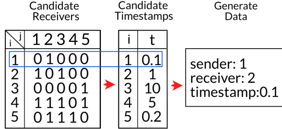
Figure 1: An illustrative example of the generative process of the HEM.
