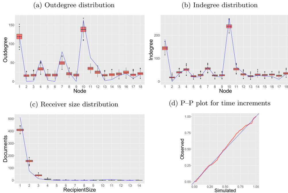
Figure 5: PPC results from log-normal distribution. Blue lines denote the observed statistics in (a)–(c) and denotes the diagonal line in (d).
