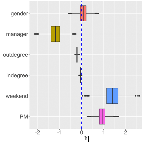
Figure 7: Posterior distribution of \eta estimates.
