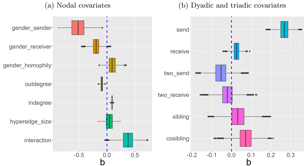
Figure 6: Posterior distribution of b estimates.
