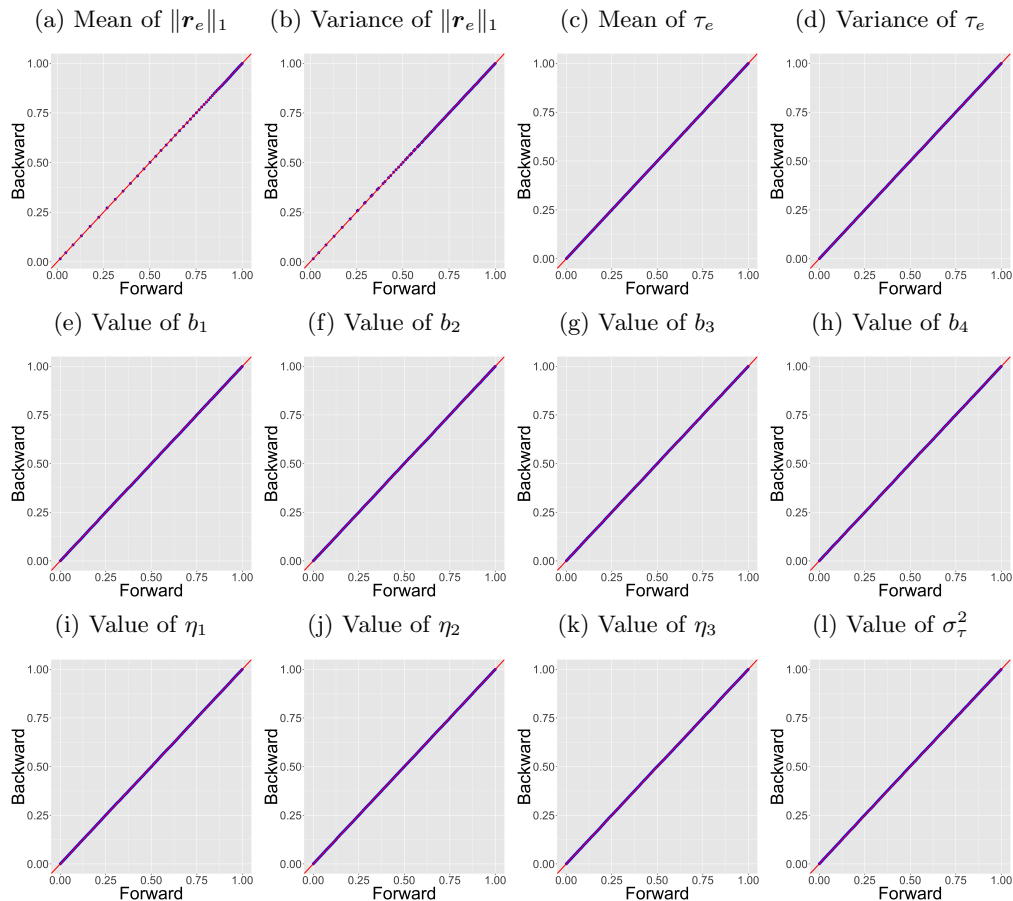
Figure 2: Probability-probability (P-P) plots for the GiR test statistics.
