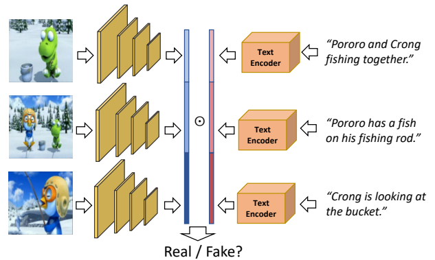
Figure 3: Structure of the story discriminator. The feature vectors of the images/sentences in the story are concatenated. The product of image and text features are input to a fully connected layer with sigmoid non-linearity to predict whether it is a fake or real story pair.
