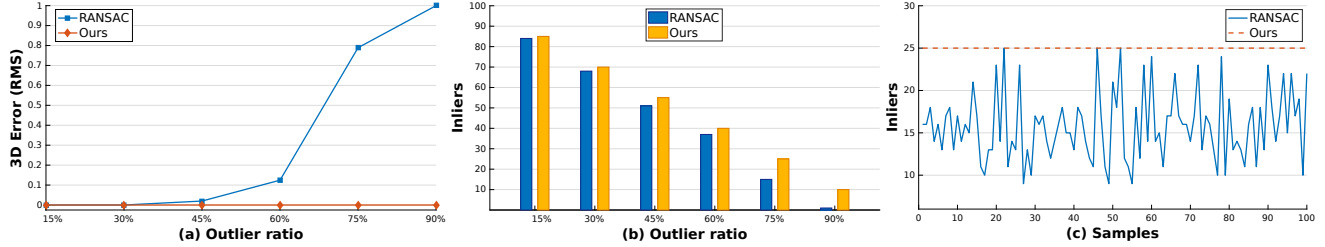
Figure 2: Similarity Transformation (synthetic data): RANSAC vs. Ours. Plots (a) and (b) show the behavior of different runs for both methods, while increasing the outlier ratio. Plot (c) shows multiple instances of RANSAC results against our method. RANSAC results in different number of inliers, while our method provides always the same exact solution.
