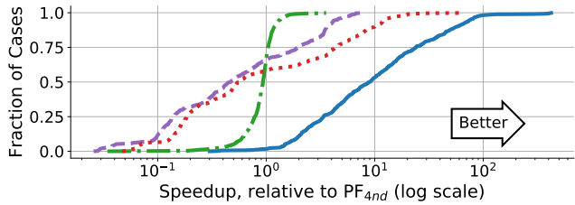
(b) CDF of speedup relative to PF_{4nd}
