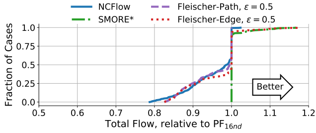
(a) CDF of total flow relative to PF_{16nd}
