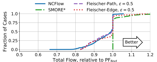
(a) CDF of total flow relative to PF_{8nd}
