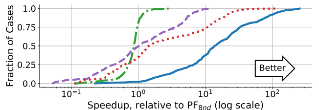
(b) CDF of speedup relative to PF_{8nd}
