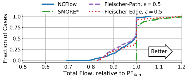
(a) CDF of total flow relative to PF_{4nd}
