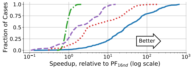
(b) CDF of speedup relative to PF_{16nd}
