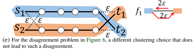
Figure 31: Alternate clustering choices that fix suboptimality concerns and disagreements.
