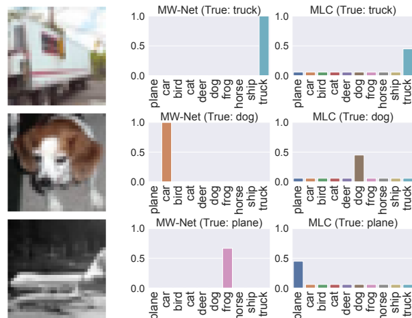
Figure 1: Illustration of label reweighting vs label correction. The first image is a truck and the given noisy label is truck, where MW-Net (A label reweighting method) and MLC successfully recover it. However, for the second image whose true label is dog and the given noisy label is automobile, MW-Net is unable to down-weight the incorrect label while MLC correctly adjusts its label by predicting the maximum weight on the class dog than all other classes. So is the case for the airplane with noisy label frog.
