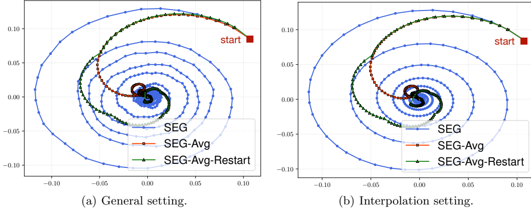
Figure 1: Illustration (in two dimensions) of the stochastic extragradient (SEG) algorithm, stochastic extragradient with iteration averaging (SEG-Avg), and stochastic extragradient with restarted iteration averaging (SEG-Avg-Restart) on the stochastic minimax optimization problem defined in Eq. (1). Here the Nash equilibrium is [\mathbf{x}^*; \mathbf{y}^*] = [\mathbf{0}_n; \mathbf{0}_m] . (a) General setting. (b) Interpolation setting, where noise vanishes at the Nash equilibrium.
