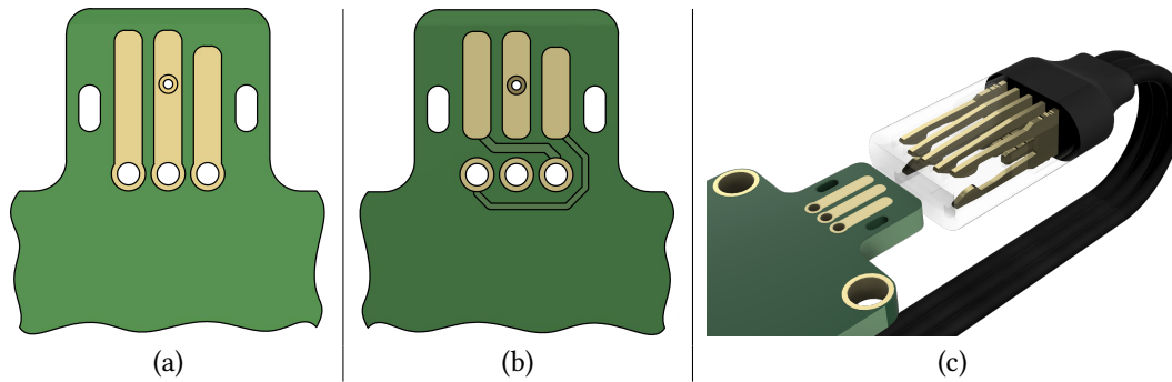
Fig. 5. PCB-based double-sided Jacdac edge and cable connectors. (a) The “top” of the edge connector has three pins, from left to right - 1) power, 2) ground, and 3) data. (b) The “bottom” of the edge connector also has three pins, from left to right: power, ground, and data - see text for more detail about wiring between top and bottom sides. (c) A 3D model of the cable connector, with housing made transparent to show internal metal fingers. See Figure 1 for photos of real examples.
