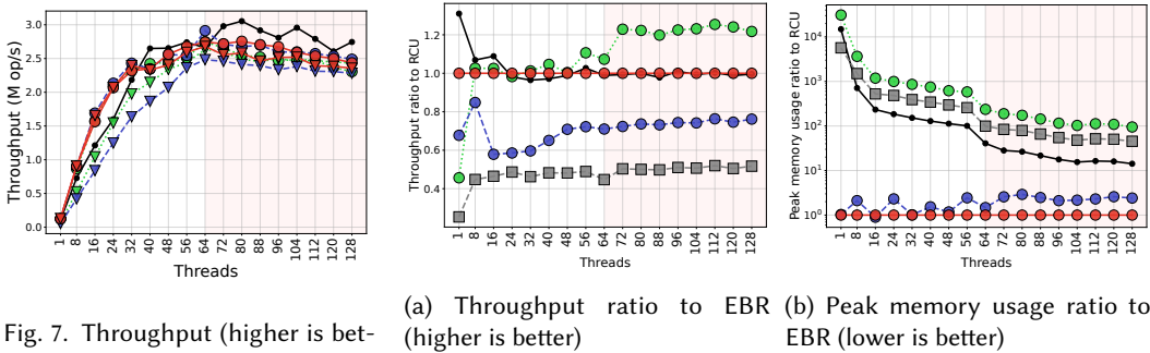
Fig. 8. DoubleLink benchmark
