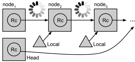
(b) After the counted reference (Rc) from node i to node i+1 is destroyed, reclaiming node i+1 requires checking its Local references, delaying its reclamation.
