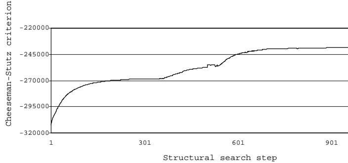
Figure 4: The Cheeseman–Stutz criterion for each intermediate model obtained during structure search when learning a three-component model for the digit “7”.
