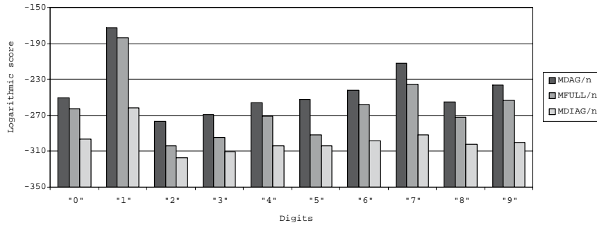
Figure 2: Logarithmic predictive scores on the test sets for the digit data.
