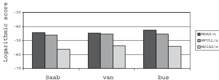
Figure 5: Logarithmic predictive scores on the test sets for the vehicle data.
