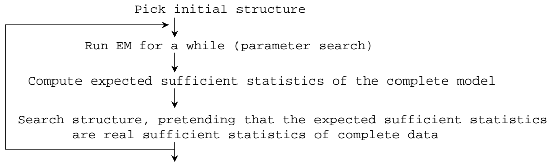
Figure 1: A schematic of our approach for MDAG model selection.
