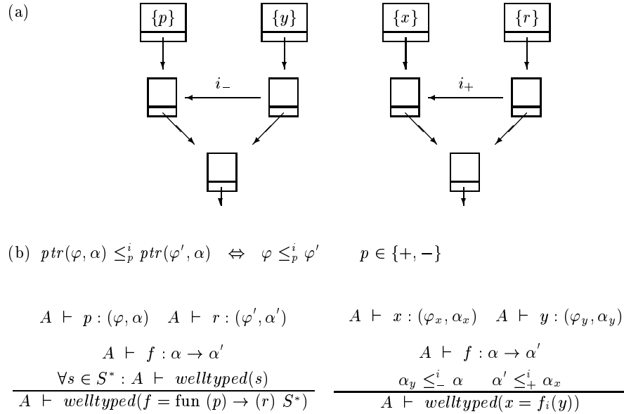
Fig. 2. Function call processing in GOLP. The graph fragments in (a) above represent points-to information after processing x = f_i(y) , a call to function f with argument y at call site i . For ease of exposition, we assume that functions are normalized: the statement f = fun(p) \rightarrow (r) S^* defines a function f that has a single formal parameter p , an out parameter r that holds the return value, and a statement body S^* . The labeled constraints \leq_-^i and \leq_+^i generated at function calls are similar to instantiation constraints used in polymorphic type inference [Hen93], except that the direction of constraints with negative ( - ) polarity is reversed to match the direction of flow of values (see [RF01]).
