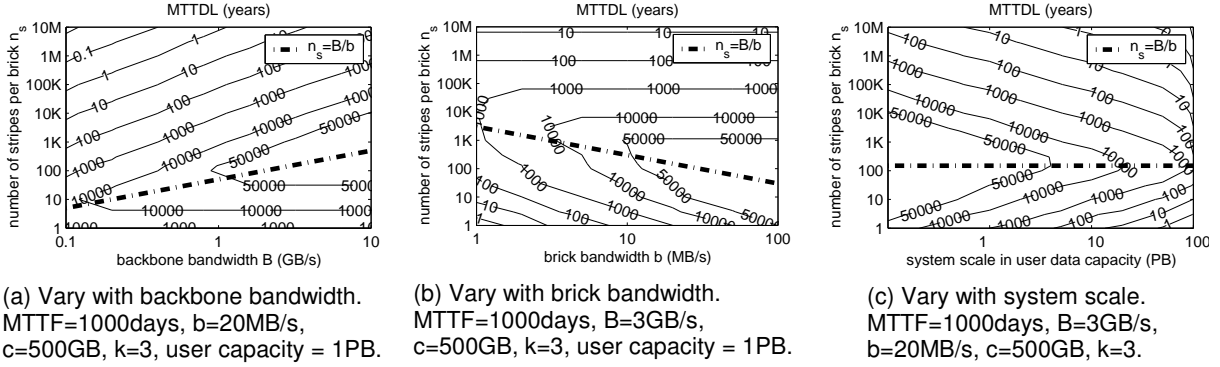
Figure 7. Contour plot for system MTTDL
