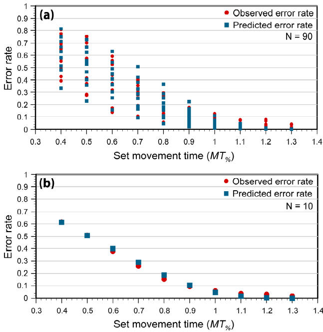
Figure 6. (a) Predicted and observed error rates for each A \times W \times MT\% across levels of MT\% . (b) Averaged over ID for each level of MT\% .
