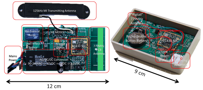
Figure 4: (left) Pulse, and (right) Link
