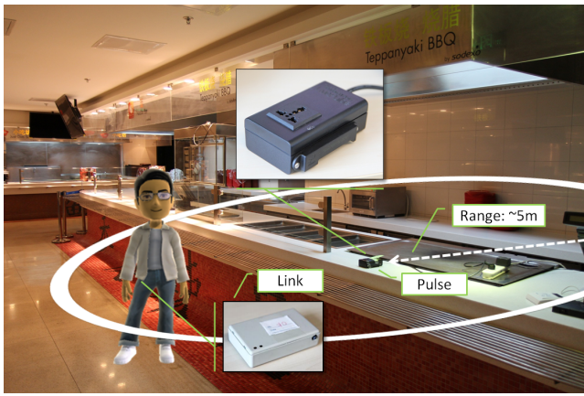
Figure 8: A Pulse is installed at the Teppanyaki counter, projecting a proximity zone of 5m radius. Links carried by diners in their pockets detect this zone as they enter.
