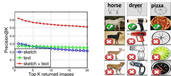
(a) Precision@K
