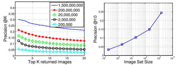
(a) Precision@K
