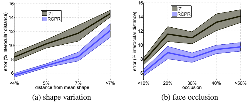
Figure 8. RCPR vs. [7] error comparison on COFW . Both average error and standard deviations are shown. (a) Error vs. increasing shape distance from average. (b) Error vs. amount of occlusion. RCPR improves [7] overall, and most significantly under high occlusions, where [7] struggles.
