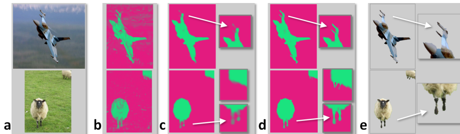
Fig. 7. The effect of contrast on thin structures. (a) Two input images. (b) unaries (from user strokes); (c) GeoS mean segmentation with no contrast. The smoothness prior makes thin protrusions (e.g. the sheep legs or the planes missiles) uncertain (grey). (d) GeoS mean segmentation with contrast enabled. Now the contrast-sensitive pairwise term correctly pulls the aeroplane and sheep thin protrusions in the foreground. (e) GeoS MAP segmentation for the contrast-sensitive energy in (d).
