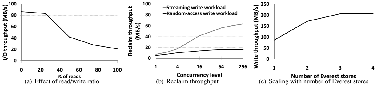
Figure 13: Micro-benchmark results.
