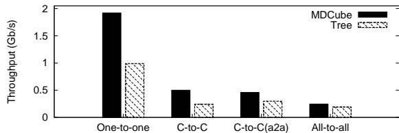
Figure 10: Per-server throughput under different traffic patterns.
