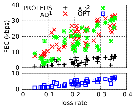
Figure 14: The FEC overhead. “OPT” shows the total FEC overhead in the optimal scenarios.
