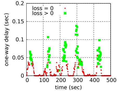
Figure 3: The one-way delay for the time windows with and without loss.
