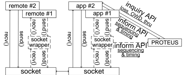
Figure 1: The overall design of PROTEUS. The details of its interaction with an application are shown in Figure 11.
