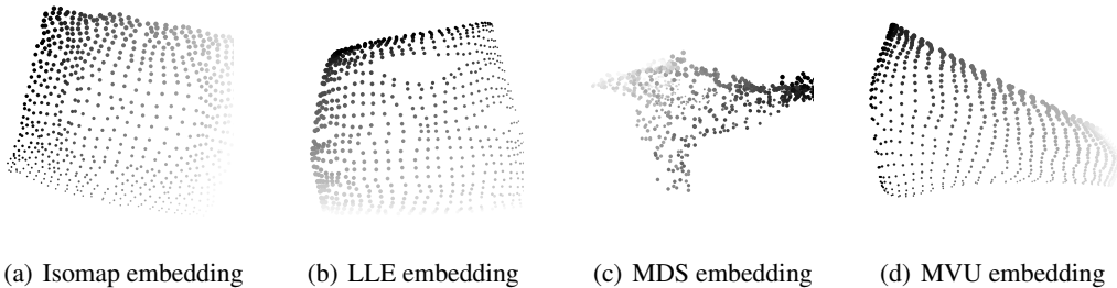
Figure 2: Examples of embeddings discovered by Isomap, LLE, MDS and MVU with 250 training images from NORB. Isomap appears most robust, and MDS the worst method, for this task.
