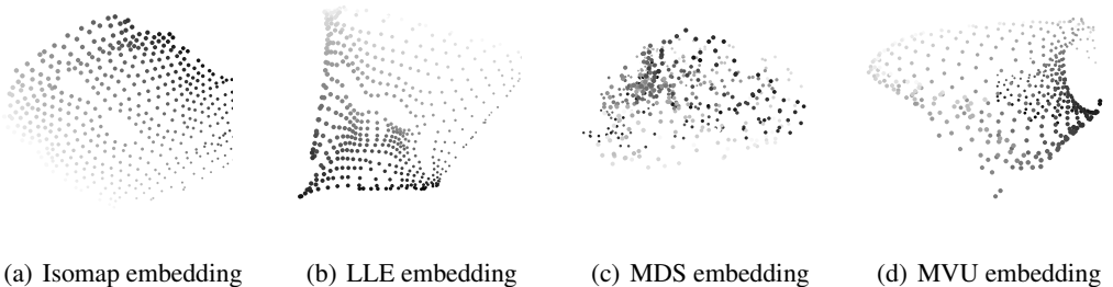
Figure 3: Examples of embeddings discovered by Isomap, LLE, MDS and MVU with 750 training images from MNIST. Isomap appears most robust, and MDS the worst method, for this task. More examples are necessary than with NORB because of the difficulty with low-variance border pixels.
