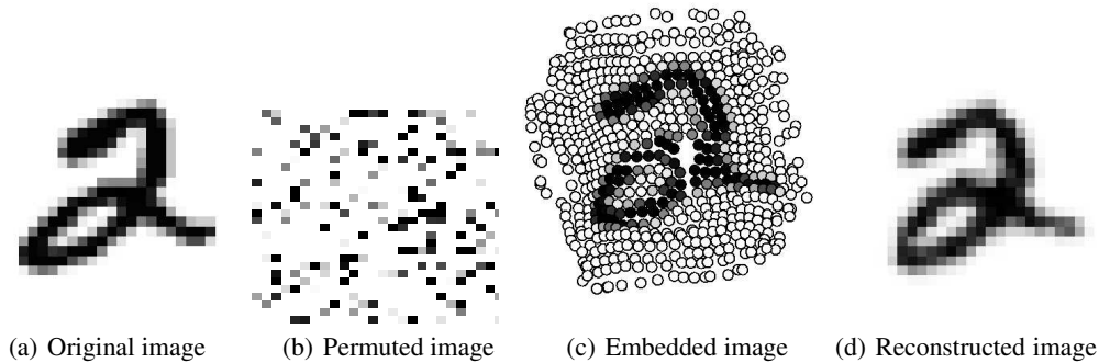
Figure 4: Example of the process of transforming an MNIST image from which pixel order is unknown (left) into its embedding (middle) and finally reconstructed as an image after rotation and convolution (right). In the middle figure we show the intensity associated to each original pixel in a circle located at the pixel coordinates discovered by Isomap.
