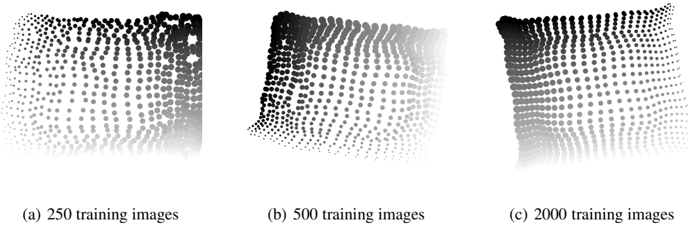
Figure 1: Embedding discovered by Isomap on the NORB dataset, with different number of training images. Each of the original pixel is placed at the location discovered by Isomap. Size of the circle and gray level indicate the original true location of the pixel. Manifold learning produces coordinates with an arbitrary rotation.
