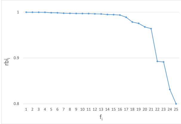
Figure 6: The real-bug indicators rbi_i for the 25 target functions f_i that lead to crashes.
