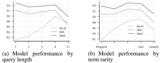
Figure 5: Performance of different models by length of query and how rare the rarest query term is in the training data. For the rare term analysis, we place all query terms into one of five categories based on their occurrence counts in the training data. Then we then categorize each query in the test dataset based on the frequency of the rarest term belongs in the query. We include a category for queries with at least one term which has no occurrences in the training data.
