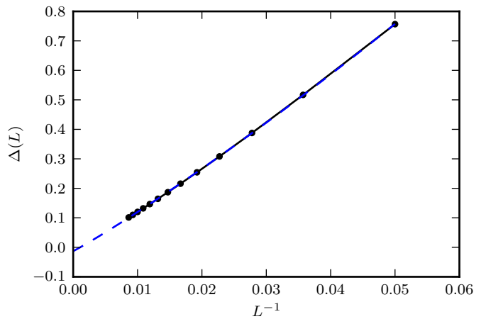
FIG. 1. Finite-system gap for the ladder with open boundary conditions. Calculations were performed with M = 1000 states. The dashed line shows a fit to Eqn. (22).
