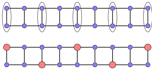
FIG. 4. Illustration of the two gapped phases. Top panel: charge ordered, Ising disordered phase. The ellipses indicate sites occupied by a fermion in the antisymmetric state (d_{i,\uparrow} - d_{i,\downarrow})|0\rangle . Bottom panel: charge and Ising ordered phase. The bigger red sites indicate occupied sites, the other sites are empty.
