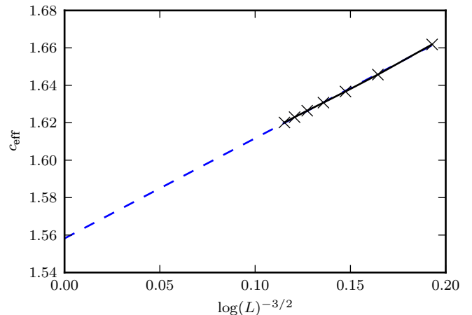
FIG. 2. Effective central charge obtained for a ladder with antiperiodic boundary conditions using M = 4800 states.
