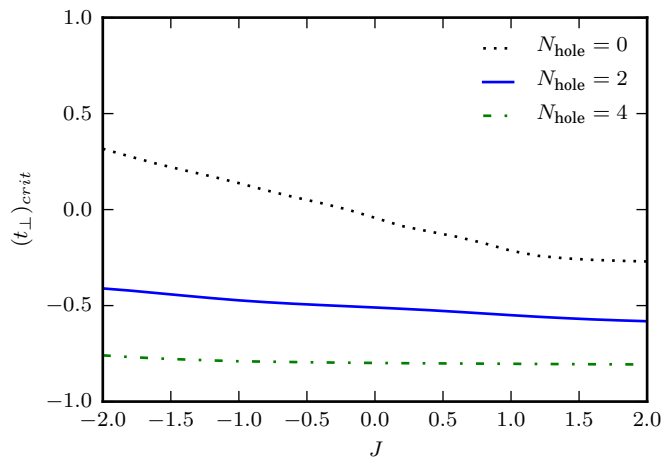
FIG. 7. Location of the Ising transition in the t_{\perp} - J phase diagram for doping away from ground state filling. The transition is determined from the peak in the central charge as t_{\perp} is varied for fixed J . Calculations are performed for L = 24 with the number of particles N = L/2 - N_{\text{hole}} .
