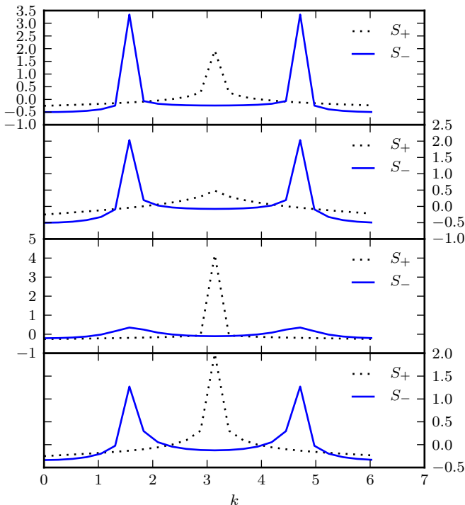
FIG. 5. Structure factor for L = 24 and antiperiodic boundary conditions. Top panel: Charge and Ising ordered phase, J = 1 , t_{\perp} = -1 . Second panel: Charge disordered, Ising ordered phase, J = -1 , t_{\perp} = -1 . Third panel: Charge ordered, Ising disordered phase, J = 0 , t_{\perp} = 0.65 . Bottom panel: Supersymmetric point.
