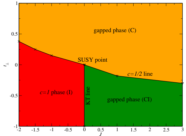
FIG. 3. Phase diagram for the model in the t_{\perp} - J plane. The labels show the shorthand notation for the phases: C corresponds to charge order, I to Ising order, and CI to charge and Ising order.
