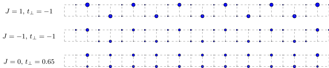
FIG. 6. Strength of the density correlation functions \langle n_{0,\uparrow} n_{j,\uparrow} \rangle and \langle n_{0,\downarrow} n_{j,\downarrow} \rangle (shown only with j > 0 ) for values of the parameters representative of the three different phases at quarter filling. The diameters of the blue, filled dots are proportional to the strength of the correlation; the upper row in each panel corresponds to \langle n_{0,\uparrow} n_{j,\uparrow} \rangle , while the lower row corresponds to \langle n_{0,\downarrow} n_{j,\downarrow} \rangle , and the distance from the left end indicates j .
