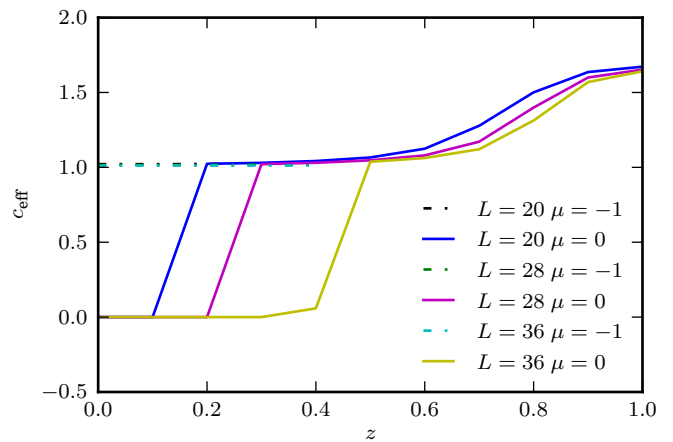
FIG. 8. Effective central charge for systems perturbed away from the isotropic supersymmetric point by staggering on two sublattices, cf. Eqn. (29). The chemical potential \mu is only added on sites on sublattice S_2 .
