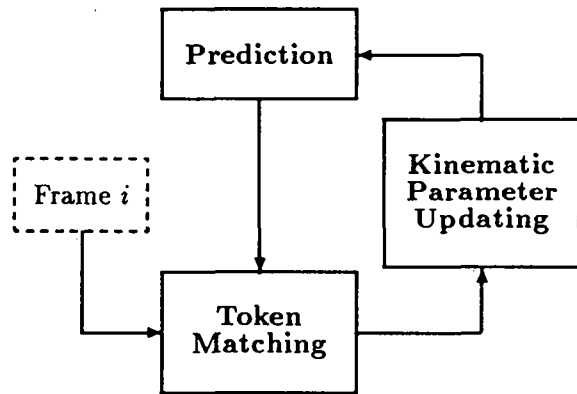
Fig. 3: Block Diagram of the Token Tracking Algorithm
